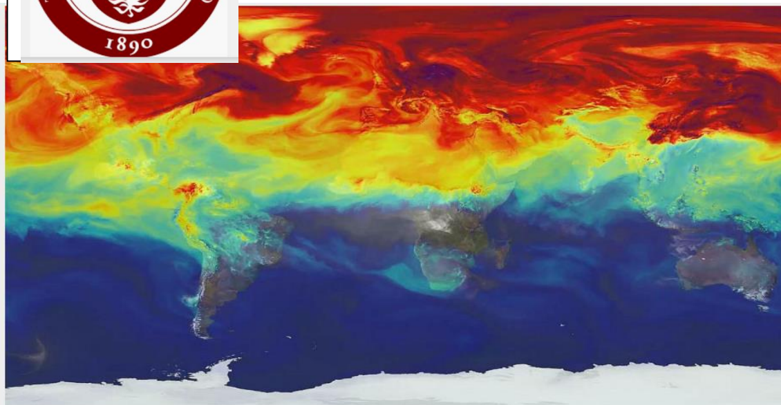
A computer simulation of carbon dioxide movement in the atmosphere.
